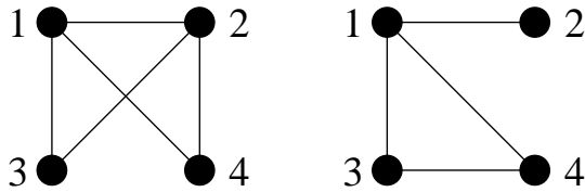
Fig. 1 Example of Local Complementation. Left: The Graph G . Right: The Graph G * 1 .
