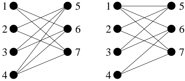
Fig. 3 Two Representations of the [7,4,3] Hamming Code. Left: The Graph G . Right: The Graph G^{(27)} .
